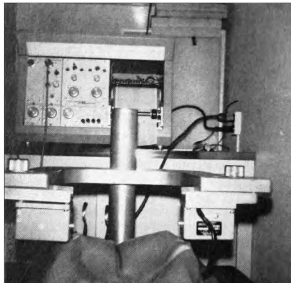
Fig. 2. Close-up of apparatus, showing pick-offs and carrying yoke.
